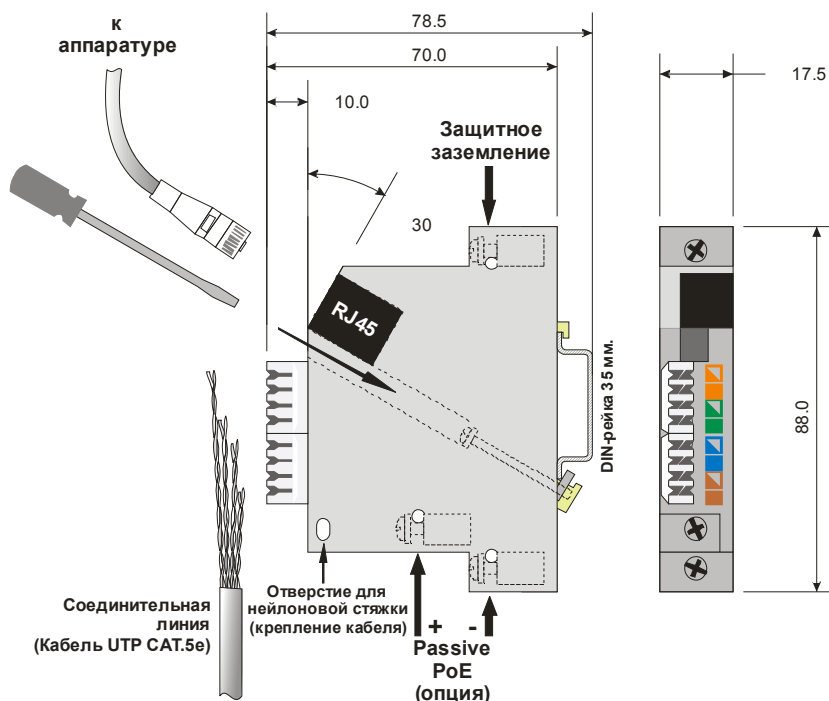
PG4PoE.x-DIN-220, PG4GPoE.x-DIN-220
